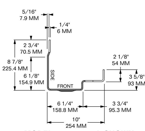
MODEL 1205-6823-L SHOWN
