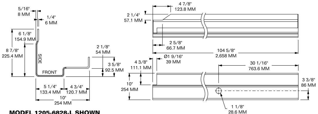
MODEL 1205-6828-L SHOWN
