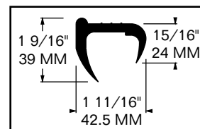
PROFILE (B)
