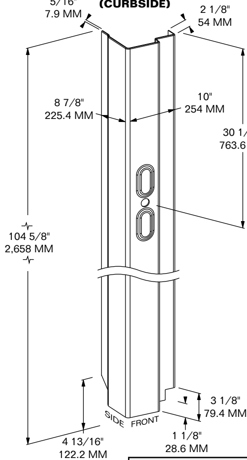
CONTAINER FRONT CORNER POST (CURBSIDE)
