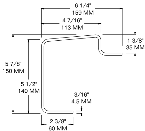
MODEL 1209-2273 REAR DOOR SILL
