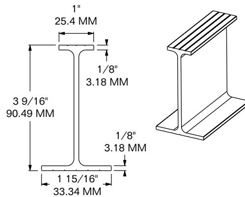
MODEL 4406-6438 PVC ROOF STRINGER
