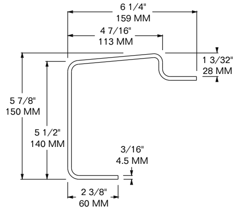
MODEL 1209-2140 REAR DOOR SILL
