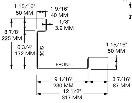
MODEL 1205-6906-L SHOWN
