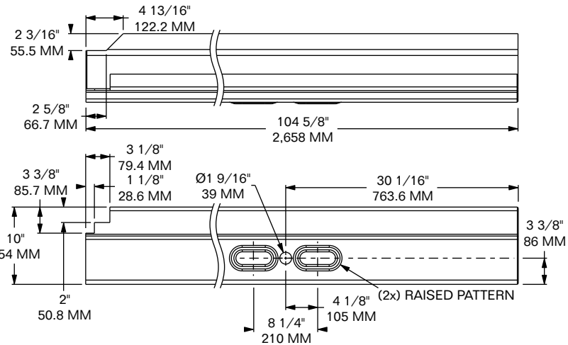
MODEL 1205-6823-L SHOWN
