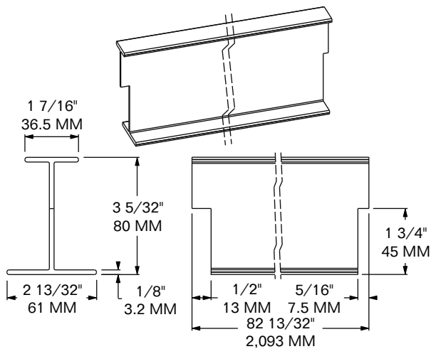
MODEL 4406-2740 PVC ROOF STRINGER
