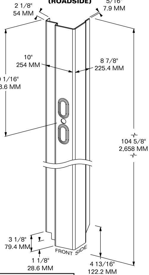
CONTAINER FRONT CORNER POST (ROADSIDE)
