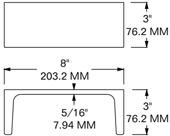
MODEL 1209-2060 C-CHANNEL INSERT
