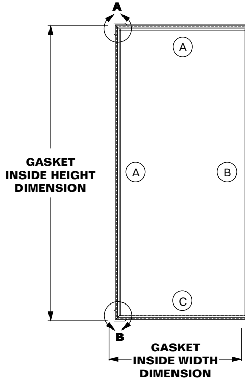
4-SIDED DOOR GASKET
